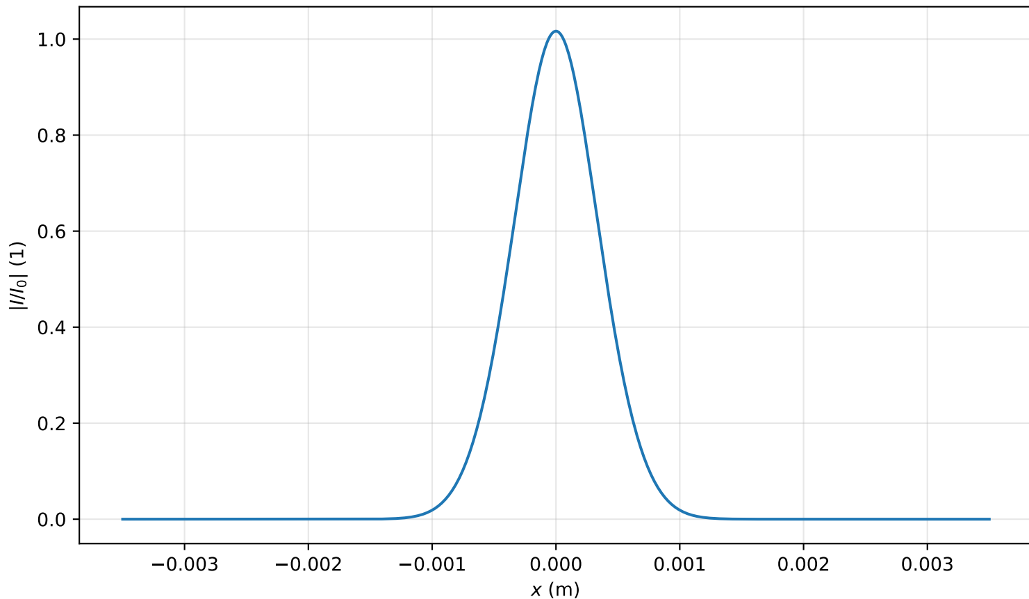
Intensity profile I(x, y = 0, z = 0.398m)/I_0 , P_{in}=0.4P_{cr} , artificial time
